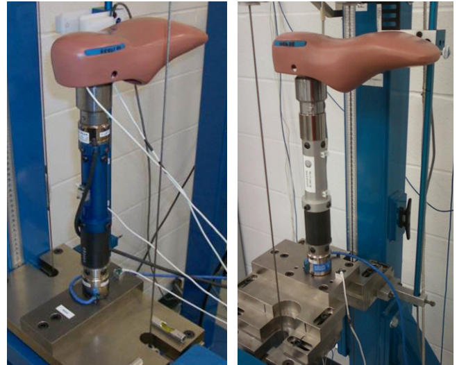
Figure 1 - Original MIL-LX test setup Figure 2 - New F-1500-0500 setup
